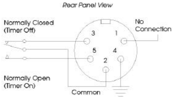
Figure 15 Timer Connections Contacts shown with TIMER OFF
