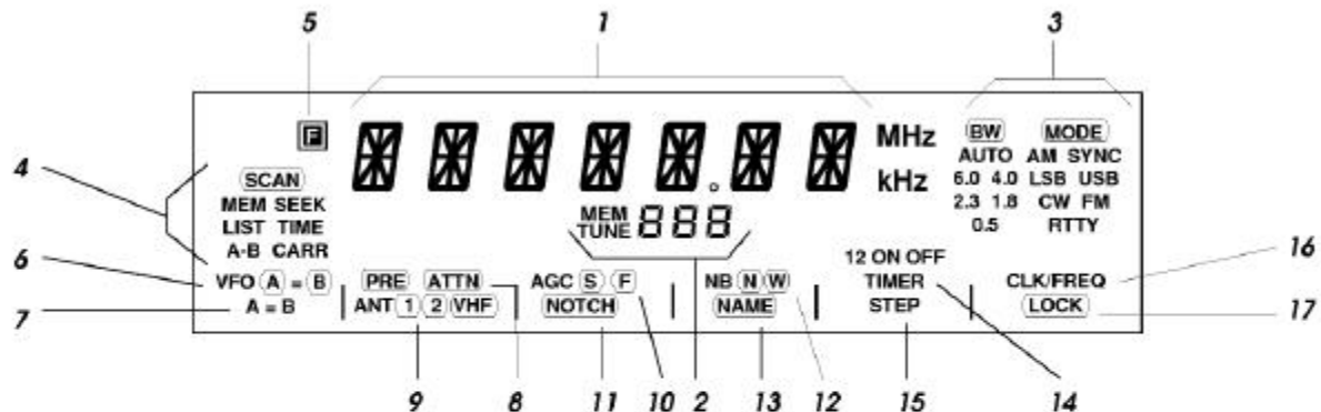
FIGURE 5 FRONT PANEL DISPLAY
