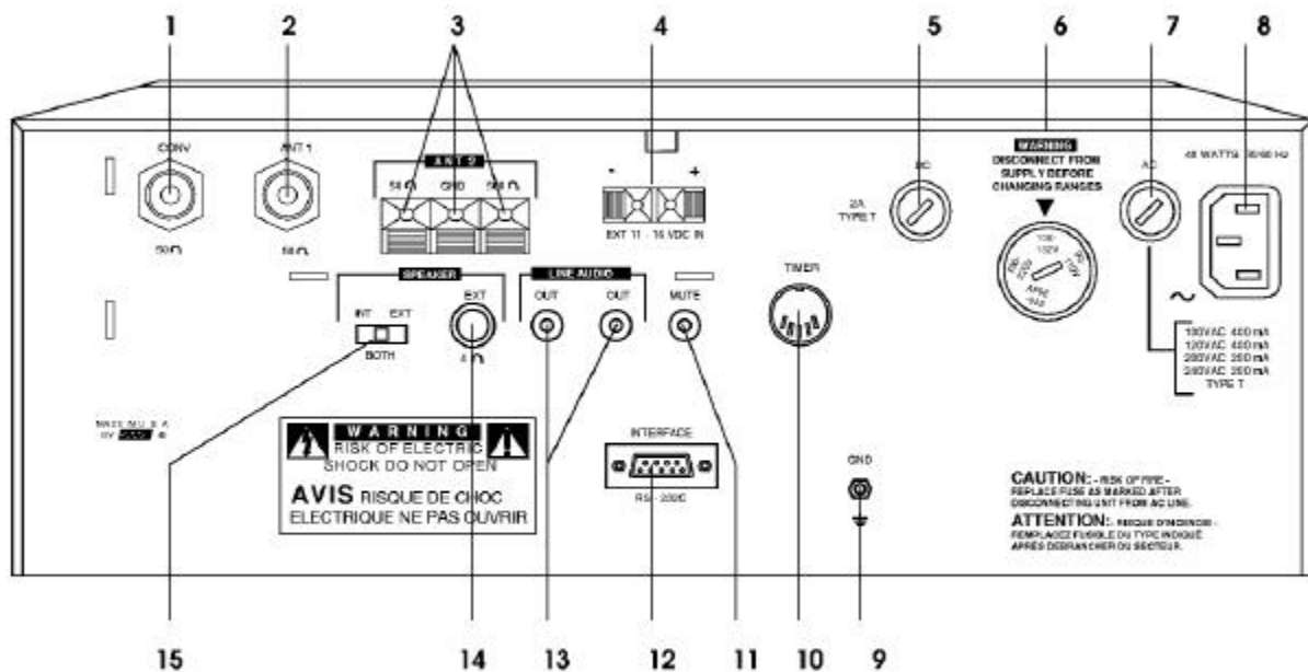
FIGURE 6 REAR PANEL
