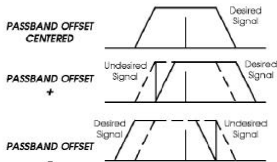
FIGURE 9 PASSBAND OFFSET Operation
