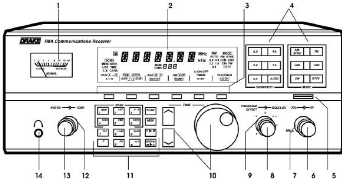
FIGURE 4 FRONT PANEL
